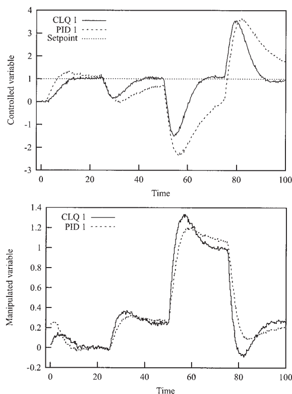
Figure 5. Integrating system: noisy case.
