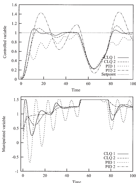
Figure 7. Underdamped system: nominal case.
